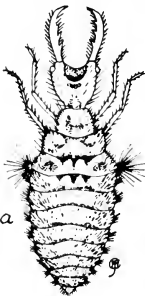
Fig. 398. a, Ant-lion, Myreleon sp.; b, A pitfall.
